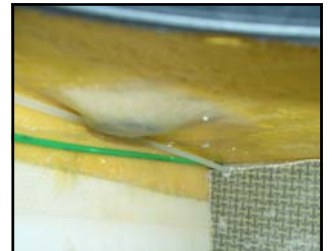
Example of pipe routing through bulkhead immediately below deck
